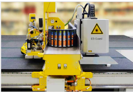
Laser marking
